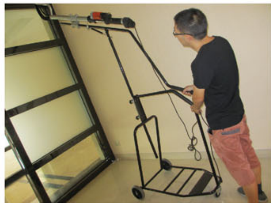
Drywall sander support cart
